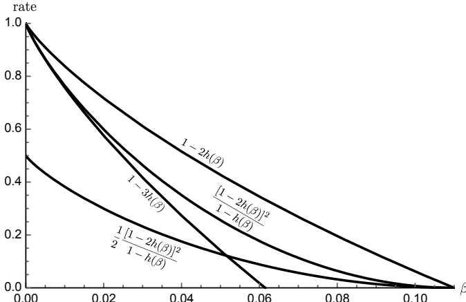
Figure 5.3: Asymptotic communication rates (4-state) as a function of the noise parameter \beta .
